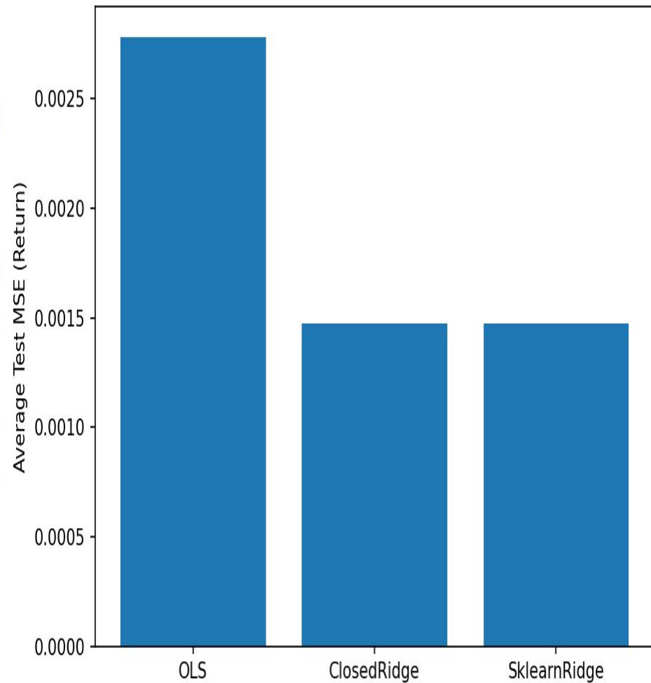
Average Return MSE by Model (Walk-forward)
